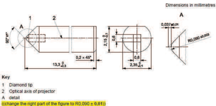
Figure 4 — Diamond scratching tip
